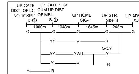
UP ASPECT CONTROL CHART →
