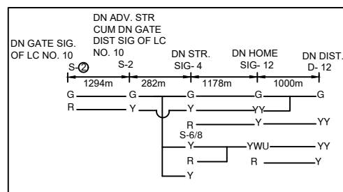
← DN ASPECT CONTROL CHART
