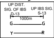
UP ASPECT CONTROL CHART FOR IBS
