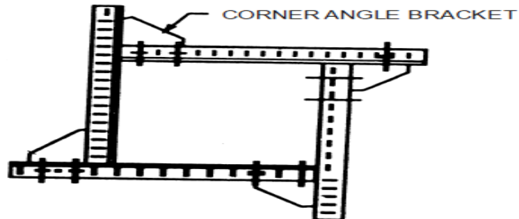
Fig. 5.6A : Four Sides Adjustable Column Form
