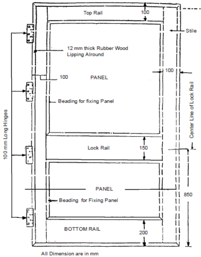
Fig. 9.16 : Typical Illustration of Panelled LVL Door Shutter
