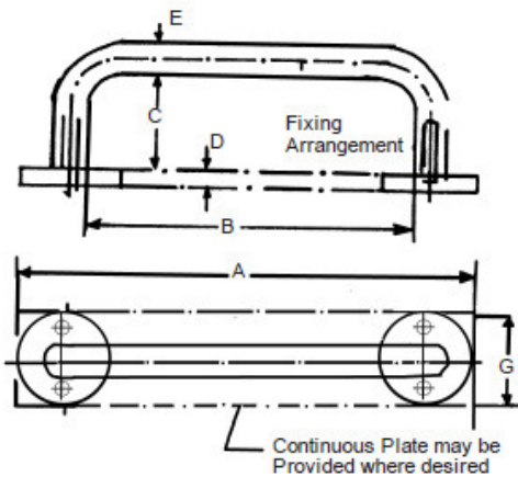
Fig. 9.12.4 : Typical Door Handle (Type 4)
