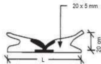
(i) METAL TIE
