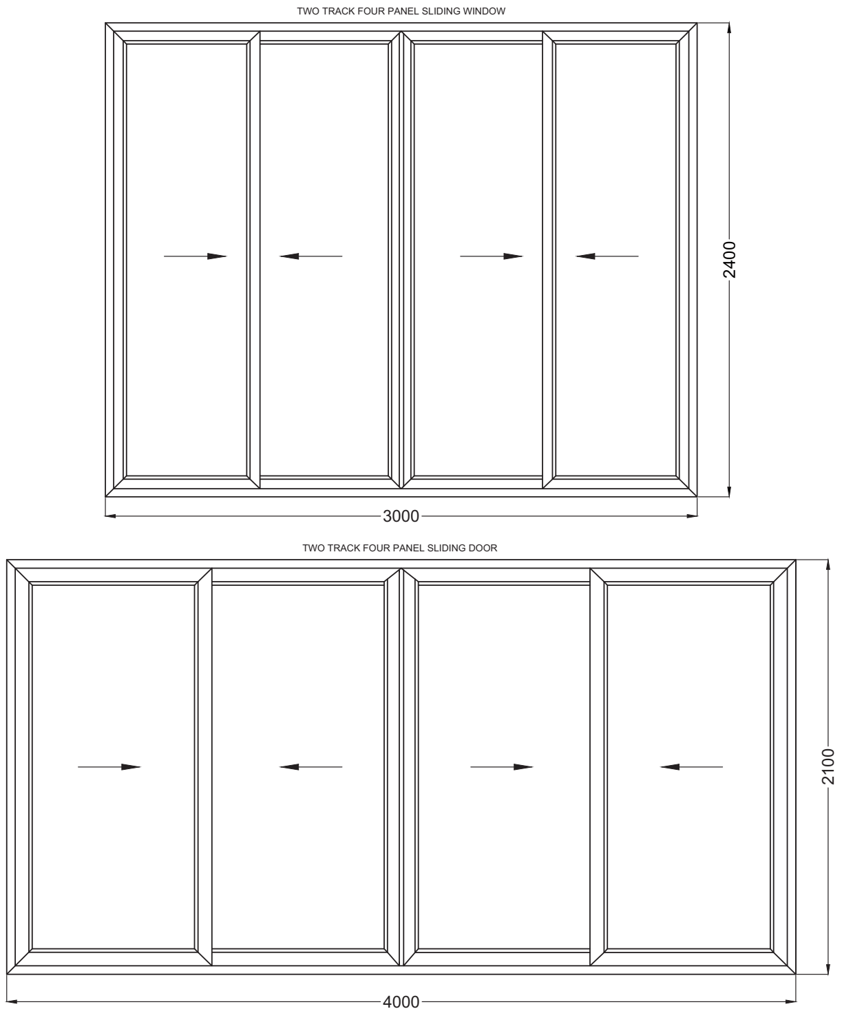
Fig. 9.33: uPVC Doors and Windows
