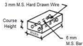
(h) BONDING UNIT (Preferably Precast R.C.C.)
