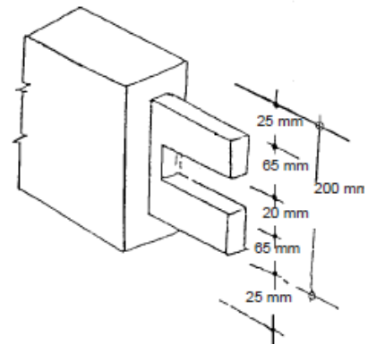
Fig. 9.16B : Double Tenon Joint
