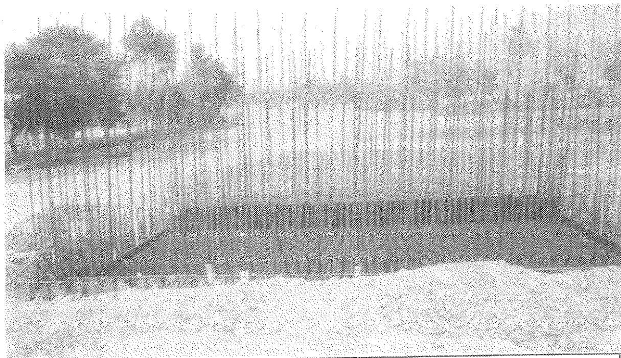
Construction of Major Bridge in Progress
