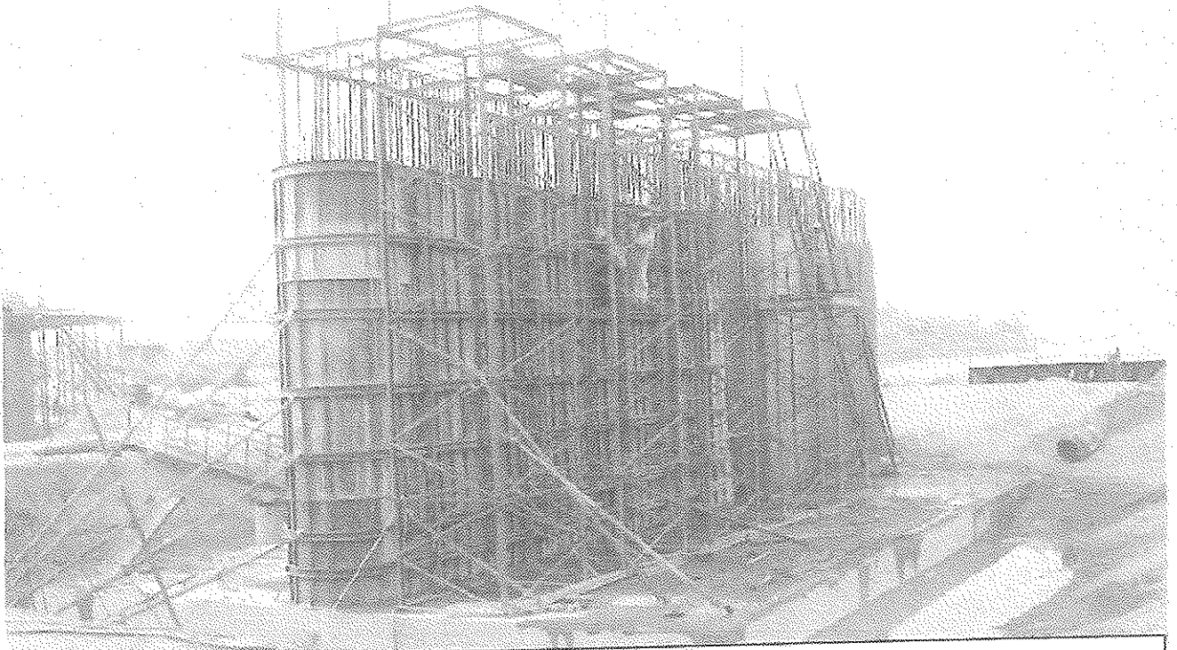
Form Work for Casting of Pier Wall
