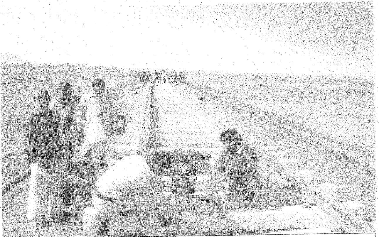
Track Linking in Progress
