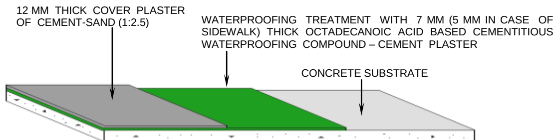
SCHEMATIC VIEW
