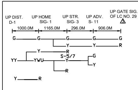
UP ASPECT CONTROL CHART →
