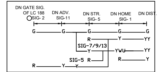
← DN ASPECT CONTROL CHART
