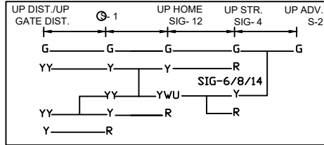
UP ASPECT CONTROL CHART →
