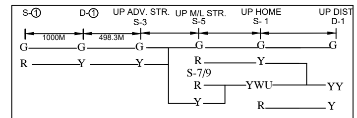
← UP ASPECT CONTROL CHART
