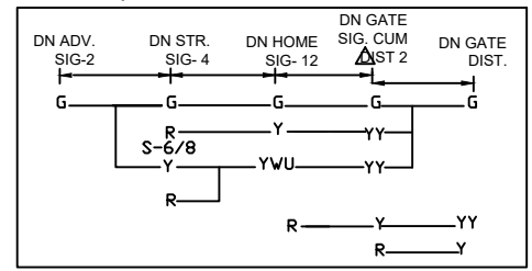
DN ASPECT CONTROL CHART
