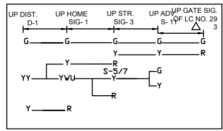
UP ASPECT CONTROL CHART
