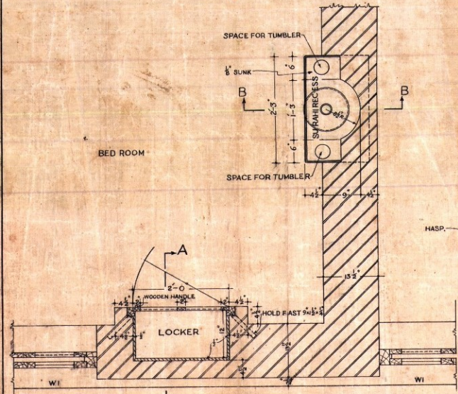
PART PLAN OF BED ROOM
